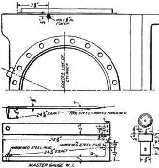
Figs. 4765-4770. Standard Datum Points, Master Gage and Tram for Valve Setting.
